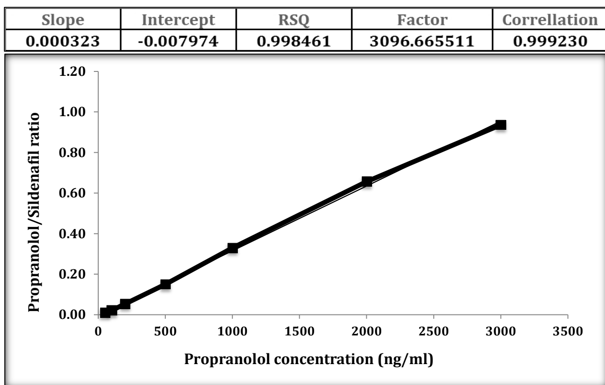
Figure 3.8 Intra-day one calibration curve of propranolol in serum.
